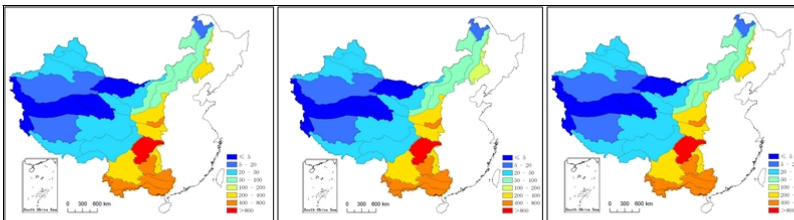
Figure 5.18. Population carrying capacity under well-off living standard (person/ km²)
