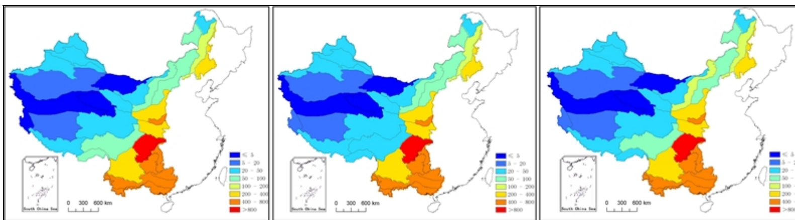
Figure 5.17. Population carrying capacity under living standard of adequate food and clothing (person/km²)
