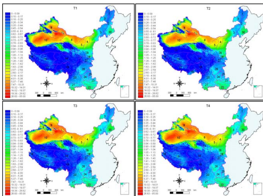
Figure 5.5. Potential evapotranspiration ratio based on HadCM3 A1FI
